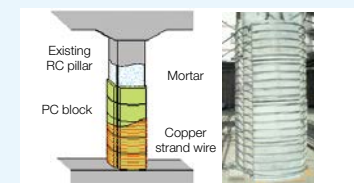
Seismic retrofitting for pillars supporting elevated tracks
